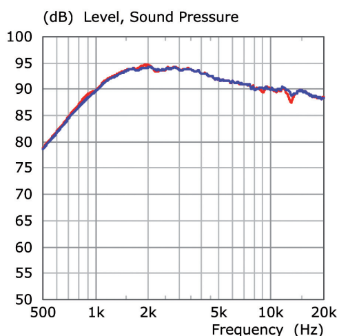
Figure 16 Actual tweeter response — Original — With cavity damping
