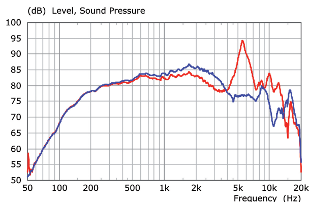
Figure 19 Response of midrange driver measured without crossover in 2π baffle — without interface — with interface
